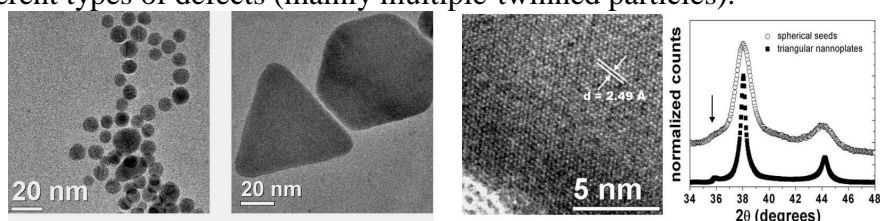
Figure 1. (from left to right) TEM images of Ag seeds; TNP formed by photochemical growth; HRTEM image of a TNP (d) XRD patterns of Ag seeds and TNPs. The arrow indicates the 2.49 Å periodicity.
